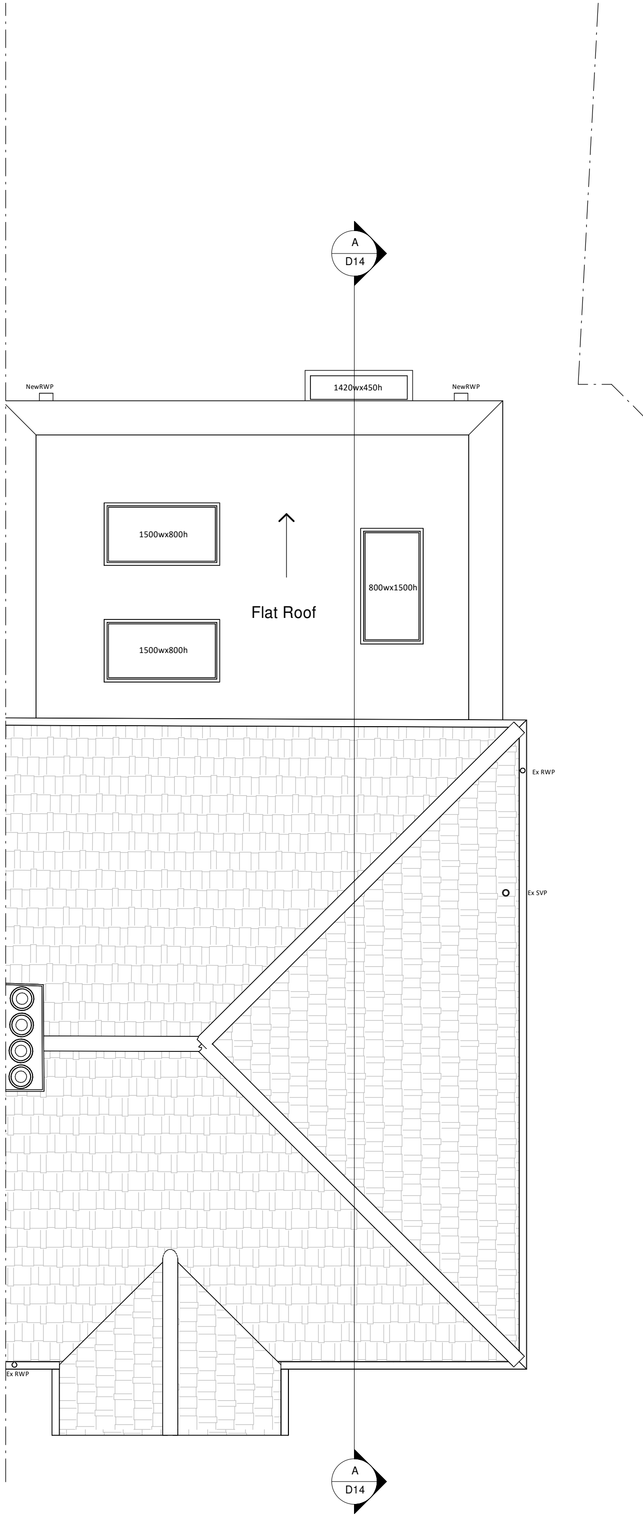
Roof Plan
