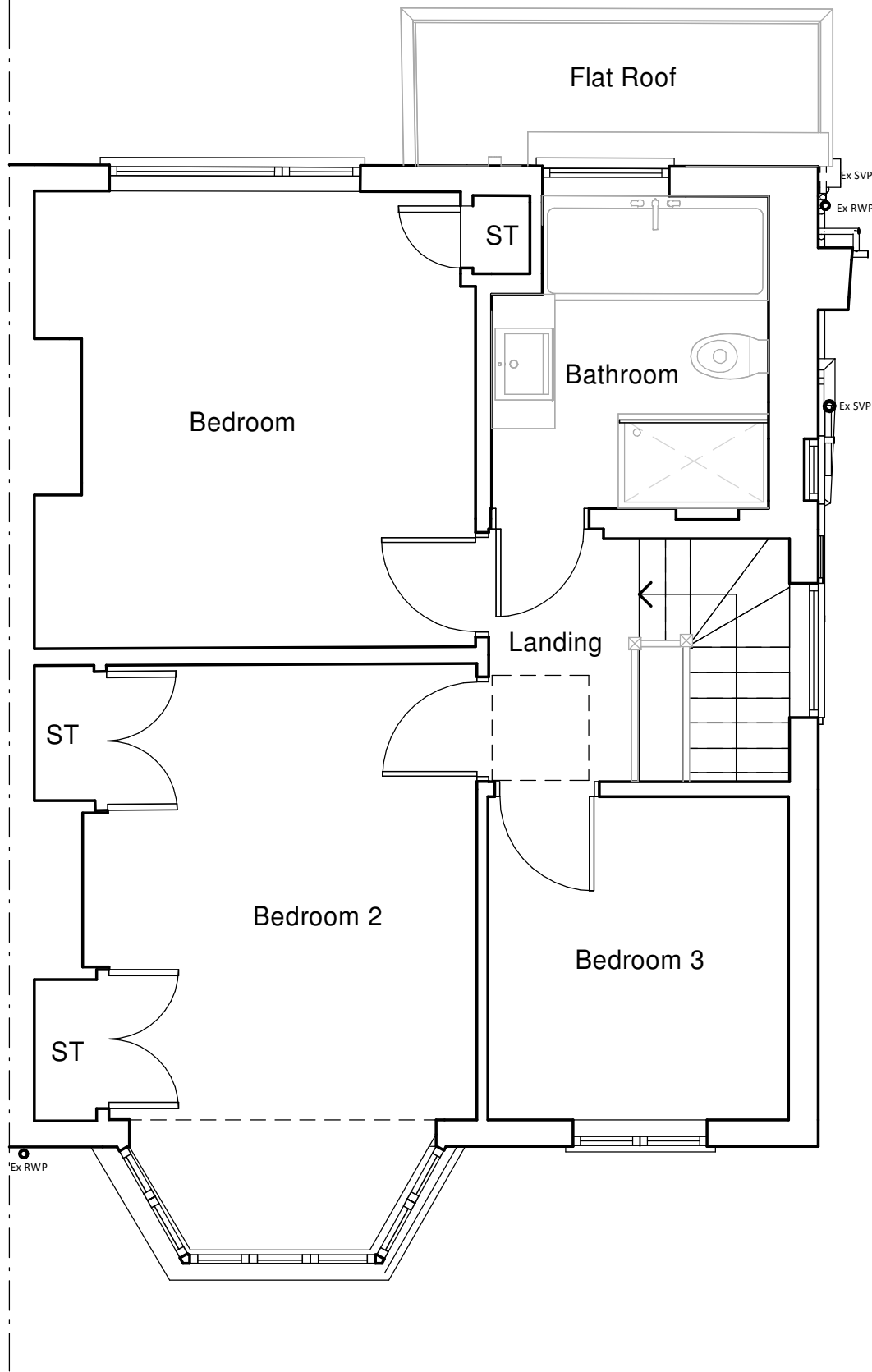
First Floor Plan Area ca. 40.68 m²
